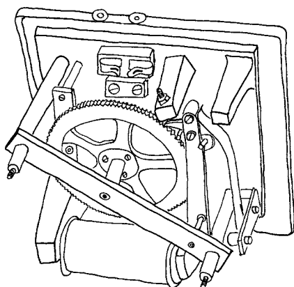
Impulse Movement Circa 1930 (Cover Removed)
