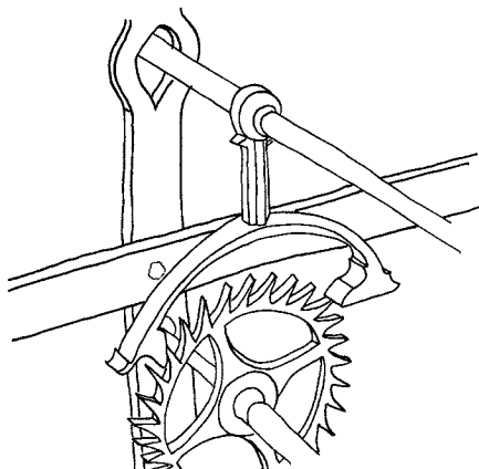
Recoil Escapement circa 1680
