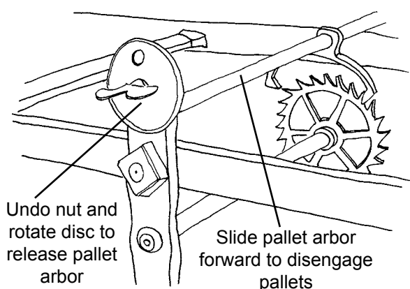
Disengaging Pallets Hand Setting circa 1700
