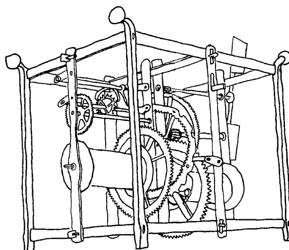
End-to-End Birdcage Movement probably 17th Century
